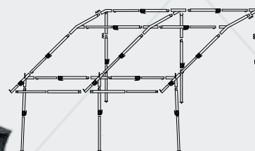
Frame diagram
